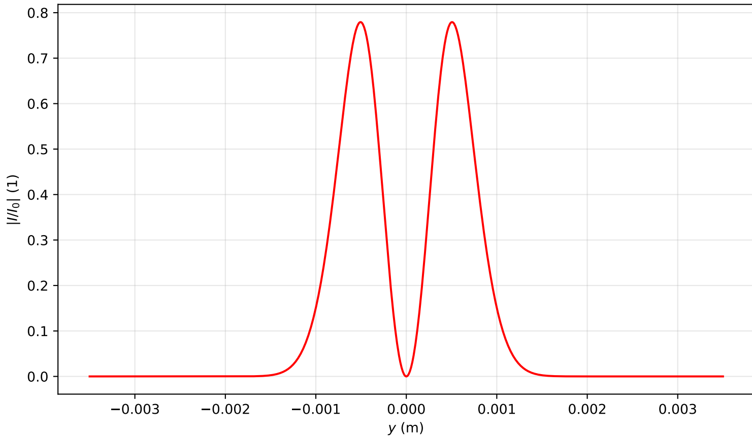
Intensity profile I(x=0, y, z=0.398)/I_0 , P_{in}=1.0P_{cr} , artificial time
